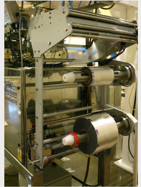
Reduce setup times with film splicing, film reel runout device and easy thread film path
